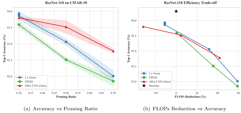
Fig. 9 Performance comparison of ResNet-110 on CIFAR-10. GRA-CNN effectively scales to very deep architectures.
