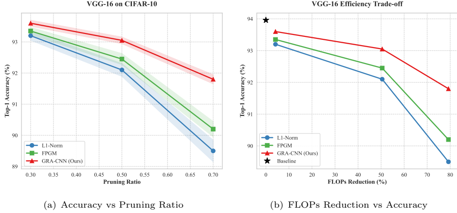
Fig. 10 Performance comparison on VGG-16 (CIFAR-10). GRA-CNN demonstrates superior generalization ability on non-residual architectures.
