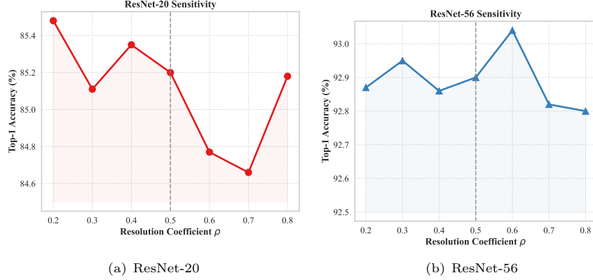
Fig. 11 Detailed sensitivity analysis of the resolution coefficient \rho . Both ResNet-20 and ResNet-56 show robust performance across a wide range of \rho values.
