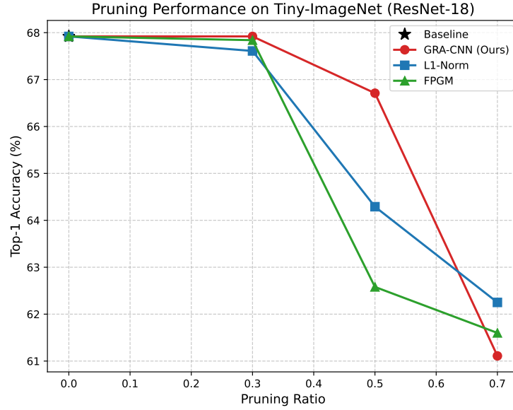
Fig. 7 Performance trajectory on Tiny-ImageNet-200 using ResNet-18. GRA-CNN exhibits superior robustness compared to L1-Norm and FPGM, particularly at the 50% pruning ratio where it maintains higher semantic fidelity.
