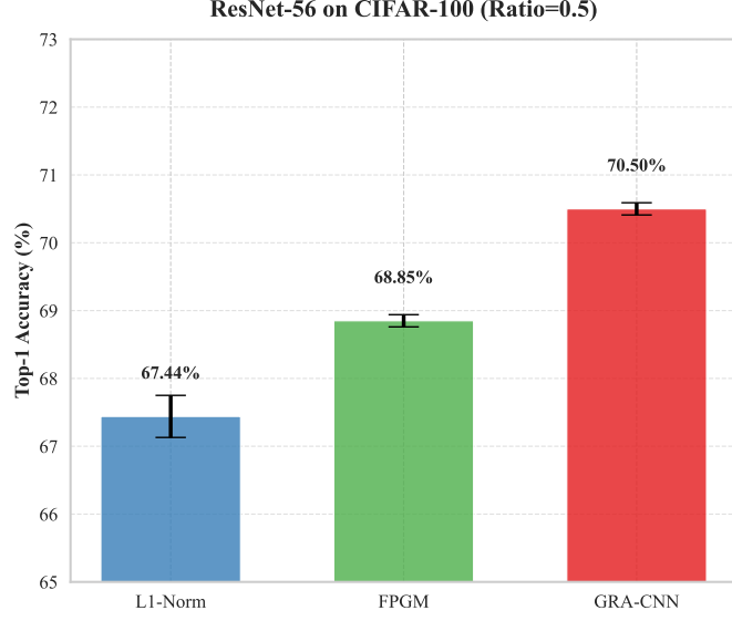
Fig. 8 Performance comparison of ResNet-56 on CIFAR-100. GRA-CNN shows superior robustness on this more challenging dataset compared to L1-Norm.
