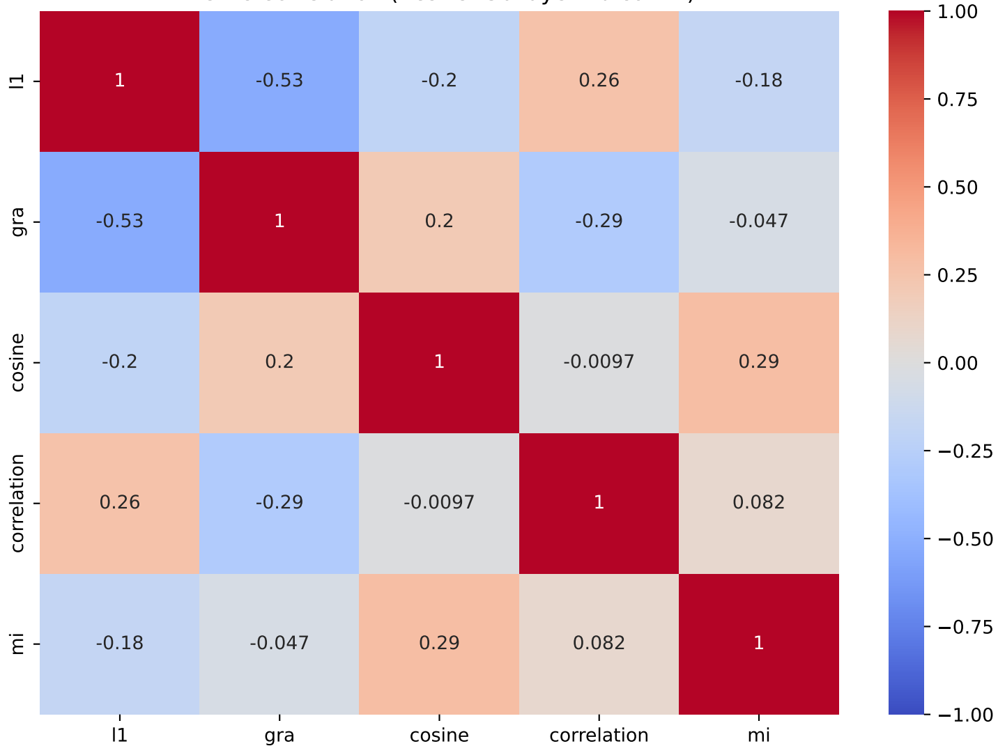
Metric Correlation (ResNet-56 layer2.0.conv1)
