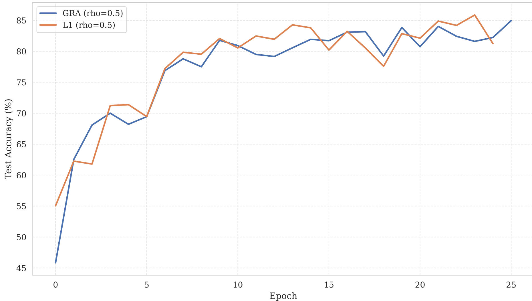
Training Convergence (ResNet-20, Ratio=0.5)
