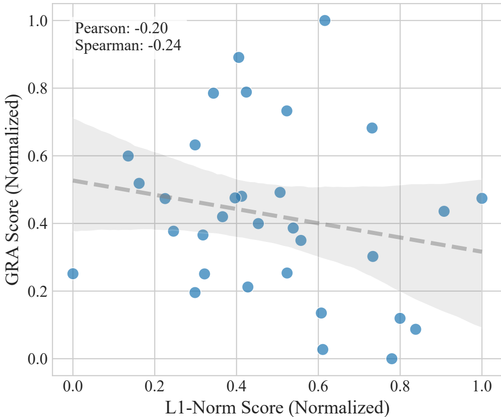
Metric Correlation (layer2.0.conv1)
