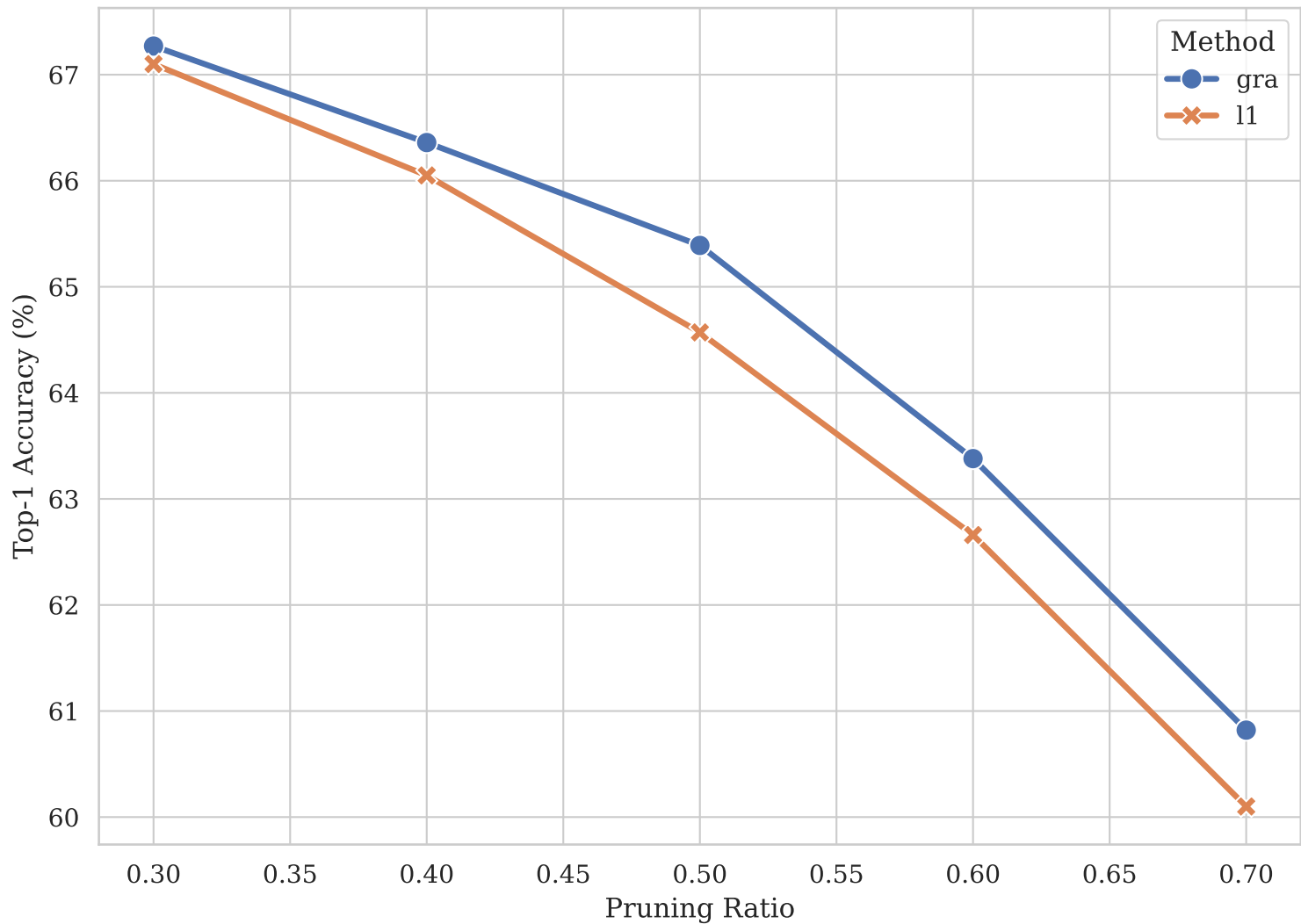
Accuracy vs. Pruning Ratio (ResNet-20 on CIFAR-100)
