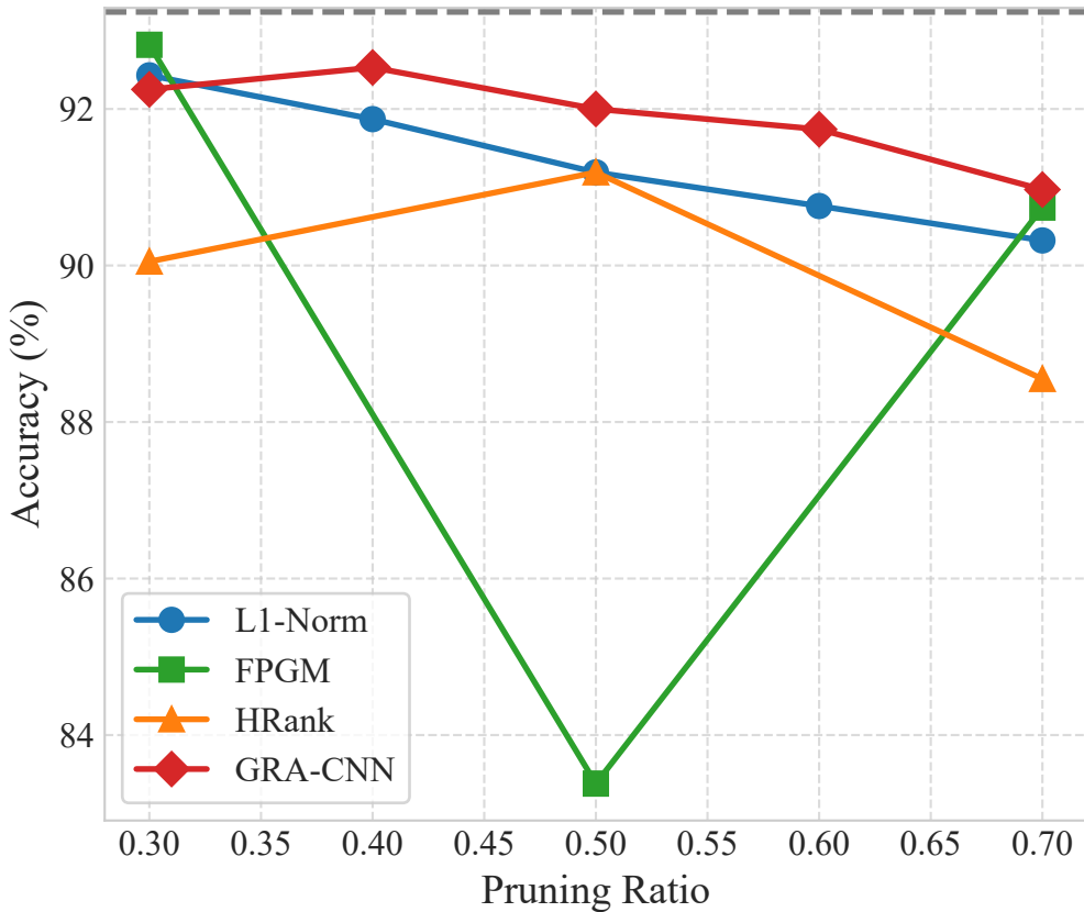
ResNet-56 on CIFAR-10
