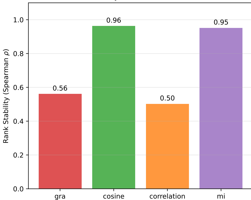
Score Stability across Different Batches
