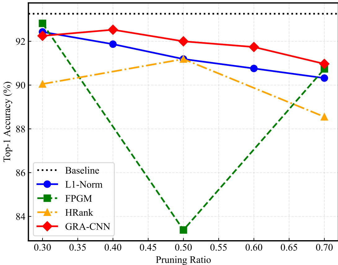
ResNet-56 on CIFAR-10
