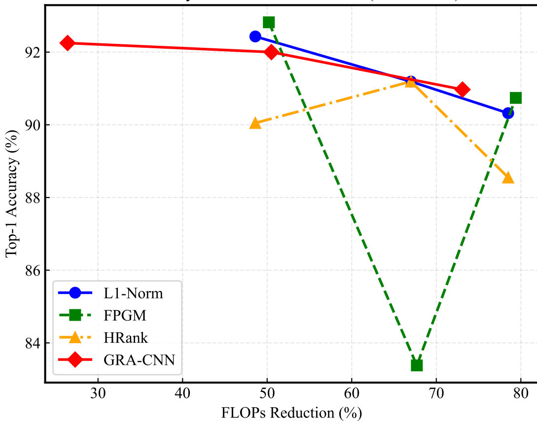
Accuracy vs. FLOPs Reduction (ResNet-56)
