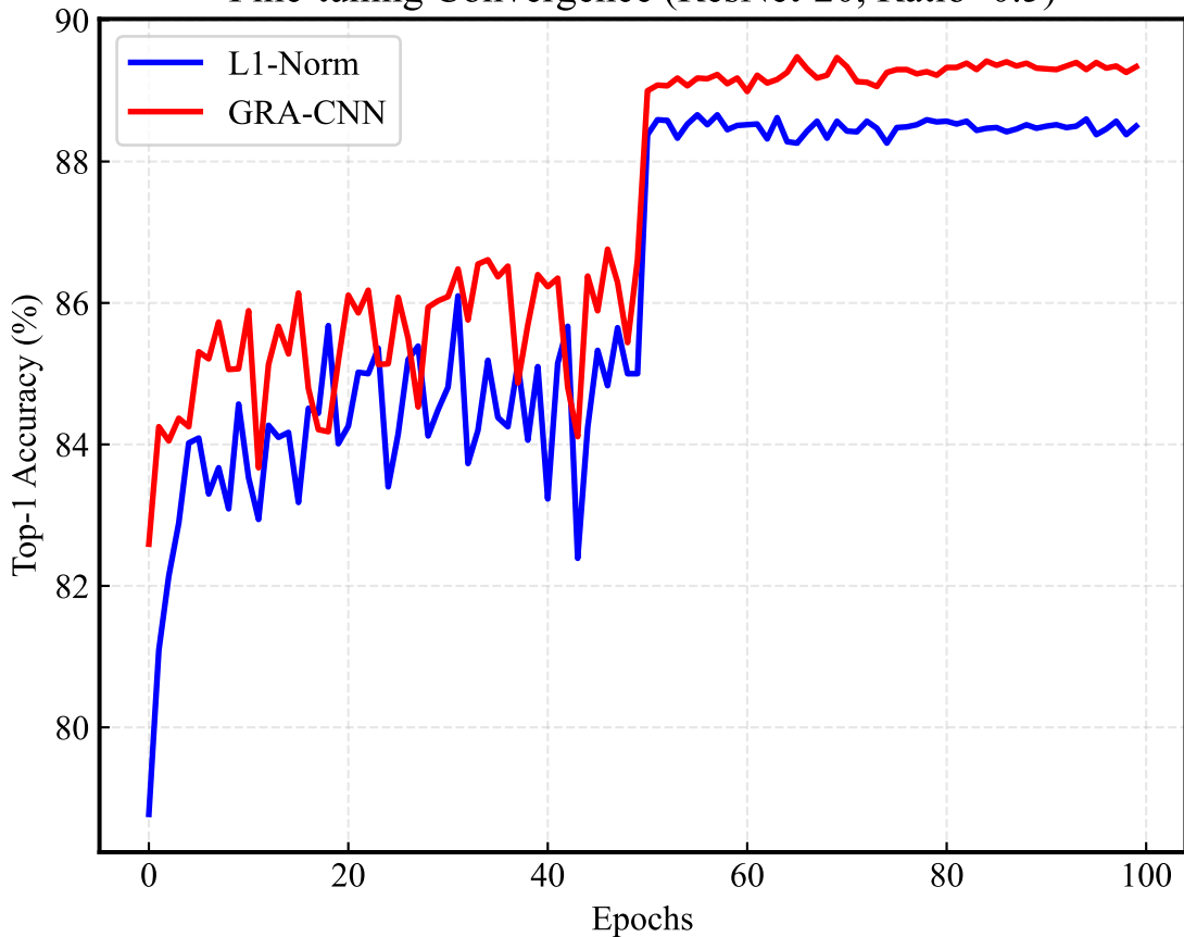
Fine-tuning Convergence (ResNet-20, Ratio=0.5)
