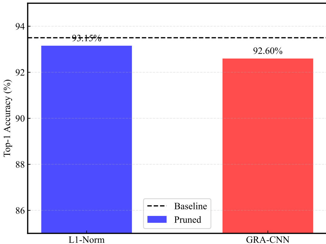
ResNet-110 on CIFAR-10 (Ratio=0.5)
