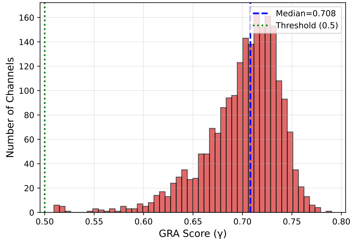
(a) Distribution of GRA Scores
