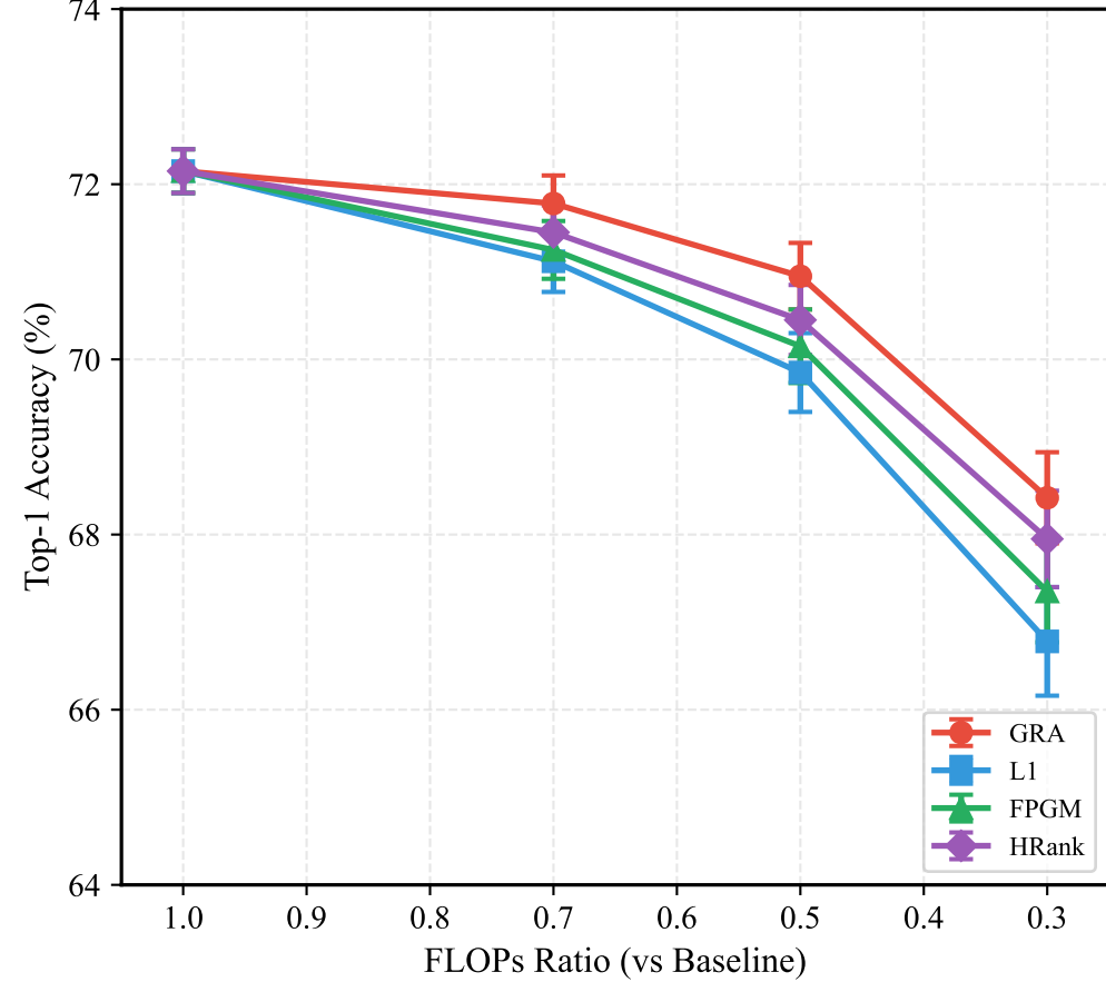
(e) ResNet-56/CIFAR-100: Accuracy vs FLOPs
