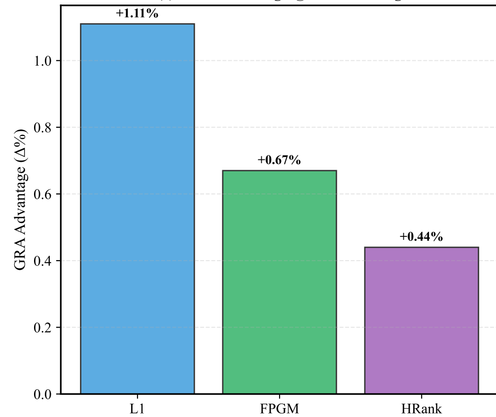
(c) GRA Advantage @ 70% Pruning
