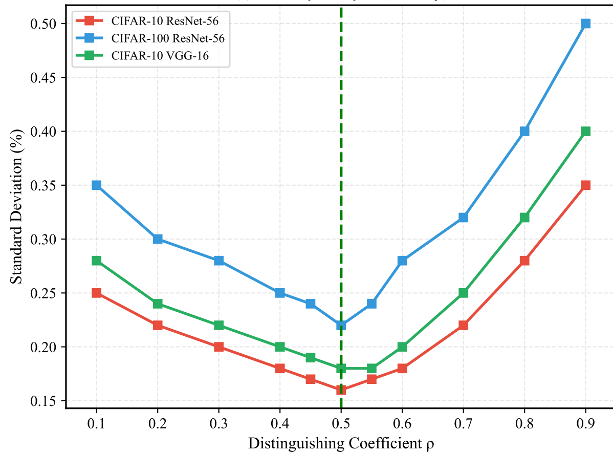
(c) Stability Analysis (Std vs \rho )
