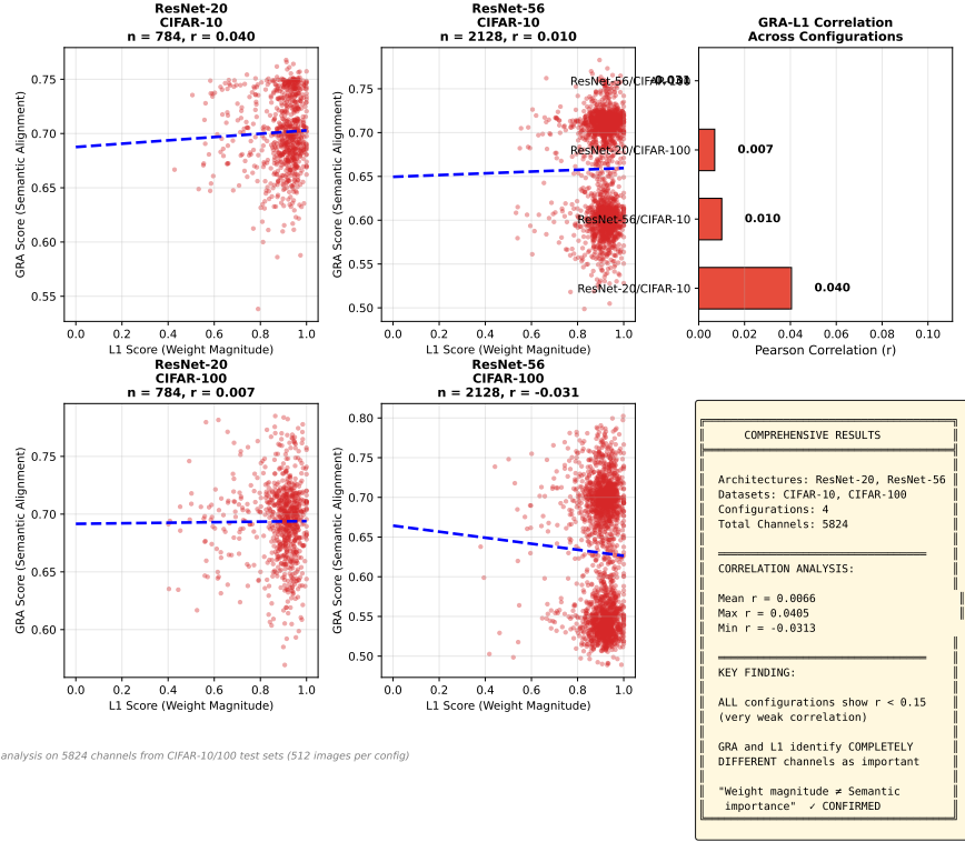
Fig. 6 Comprehensive cross-metric correlation analysis between L1-Norm (structural) and GRA score (semantic) across 4 configurations: ResNet-20 and ResNet-56 on CIFAR-10 and CIFAR-100. Each scatter plot shows all channels ( n = 5824 total). The near-zero Pearson correlation across all configurations (Mean r = 0.007 , Max |r| < 0.04 ) demonstrates that the two metrics are nearly orthogonal regardless of architecture or dataset complexity. This strongly supports our hypothesis that weight magnitude does not equal semantic importance.
