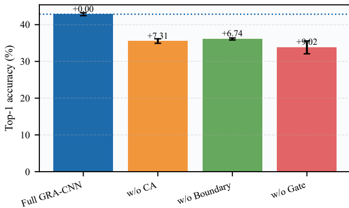
VGG-16 / p = 0.9
