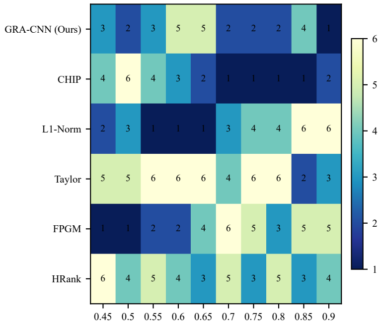
VGG-16 ranks
