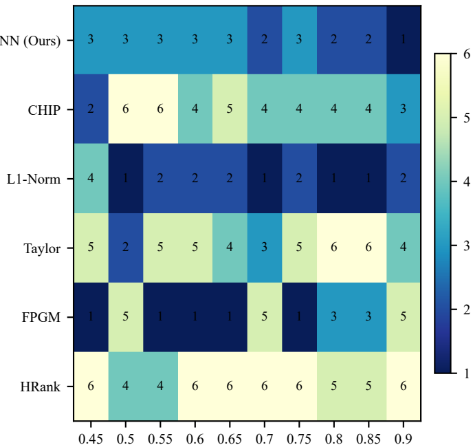
ResNet-56 ranks
