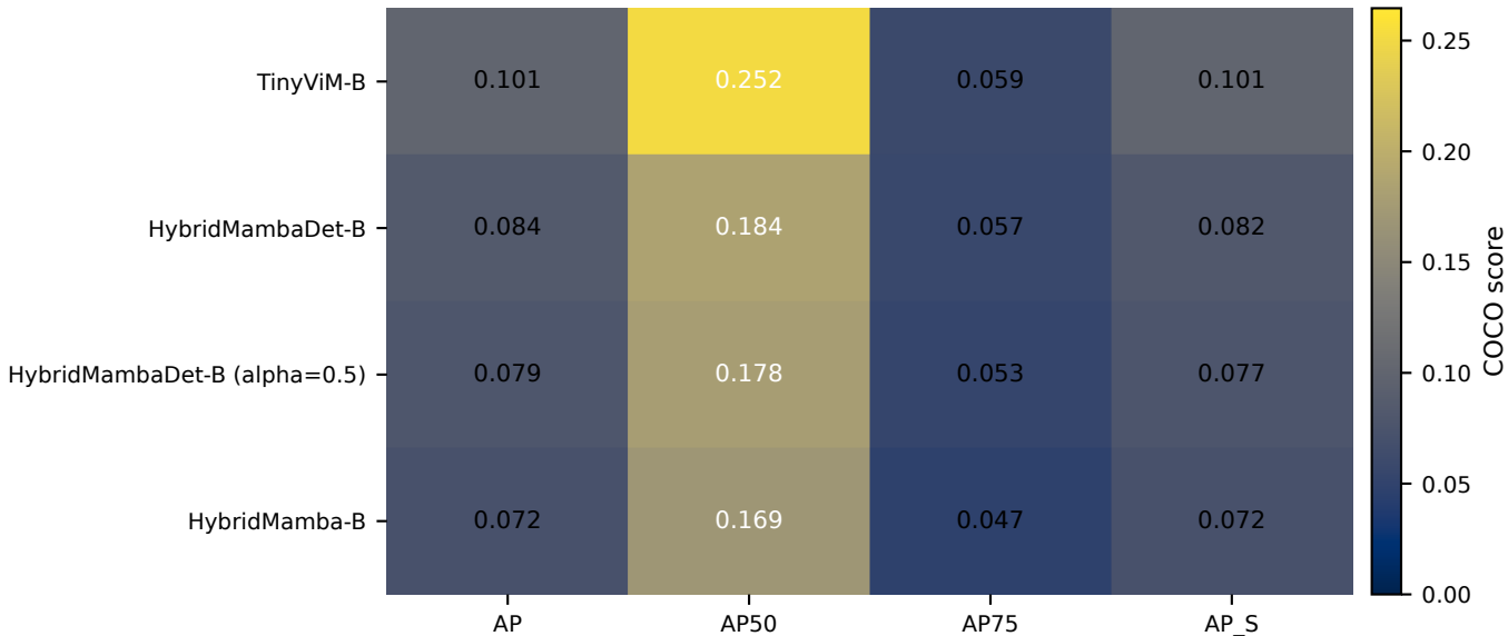
Best validation metrics by algorithm
