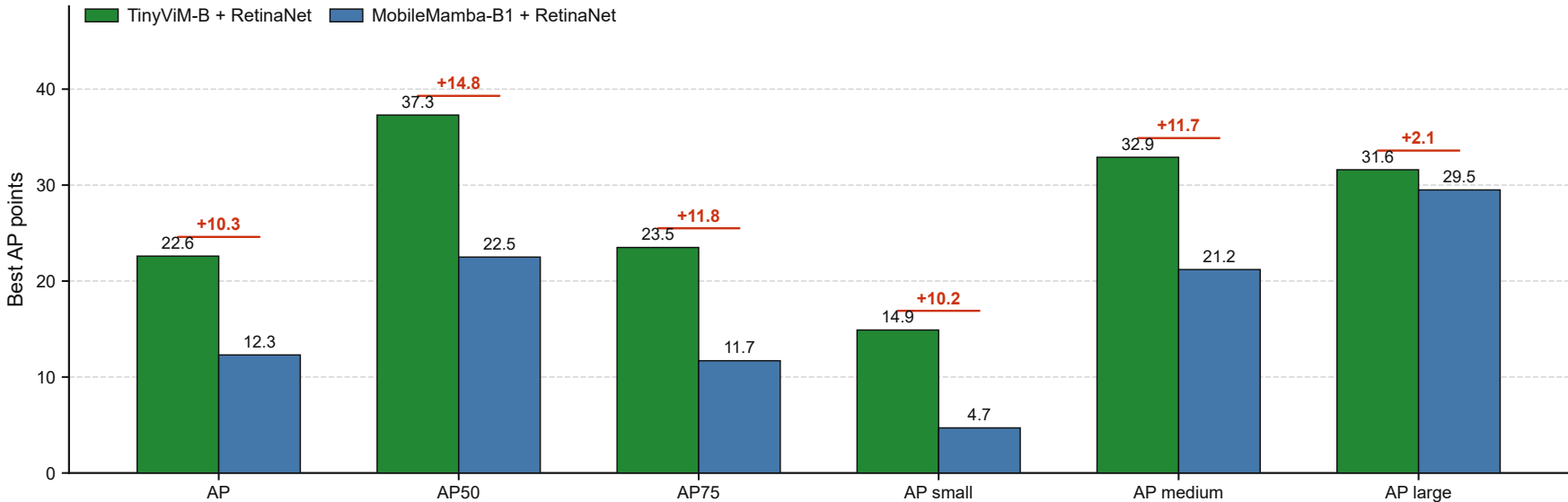
Metrics at the best-AP checkpoint favor TinyViM-B across localization and object scales
