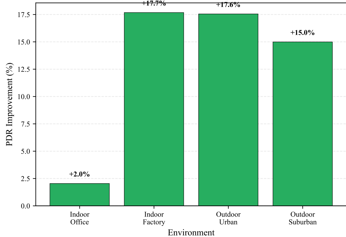
(b) PDR Gain When Gateway Disabled
