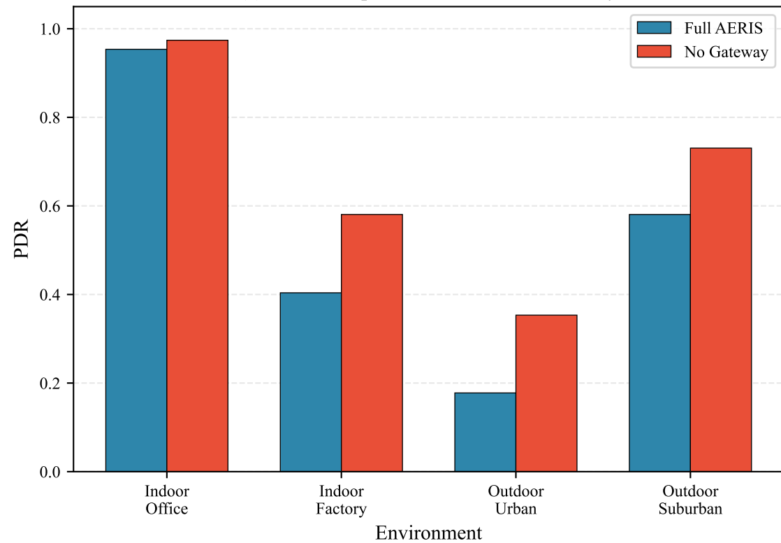
(a) PDR Comparison: Full vs No Gateway
