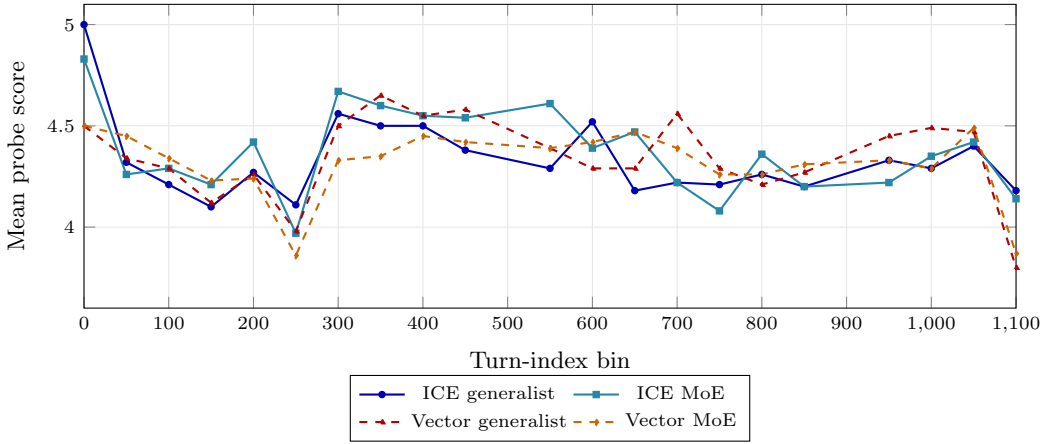
Fig. 3. Longitudinal mean score by turn-index bin (1,057 probes, Dataset C excluded; real per-bin data). The four conditions track closely mid-conversation, but at the final turn-1,100 bin—the deep long-horizon regime of Dataset B—both vector conditions drop sharply while both ICE conditions hold.
