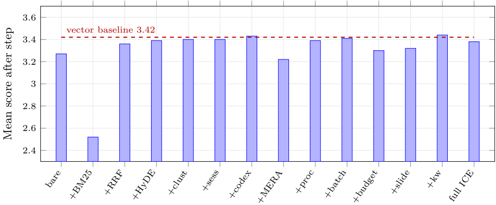
Fig. 4. Feature ablation buildup (Dataset B, 67 probes). Each bar is the cumulative mean score after adding one feature to all previous ones. The only two movements clearing a paired bootstrap CI are the +BM25 drop and the +RRF recovery. The dashed line marks the single-leg vector baseline, which is not a buildup step; the full build finishes level with it.
