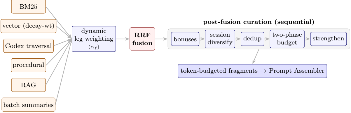
Figure 2: Retrieval orchestrator. The legs are heterogeneous in retrieval semantics; RRF is what allows them to be combined without score normalisation; the two-phase budget guarantees leg diversity under budget pressure. Section 8.1 reports which legs contributed during evaluation.
