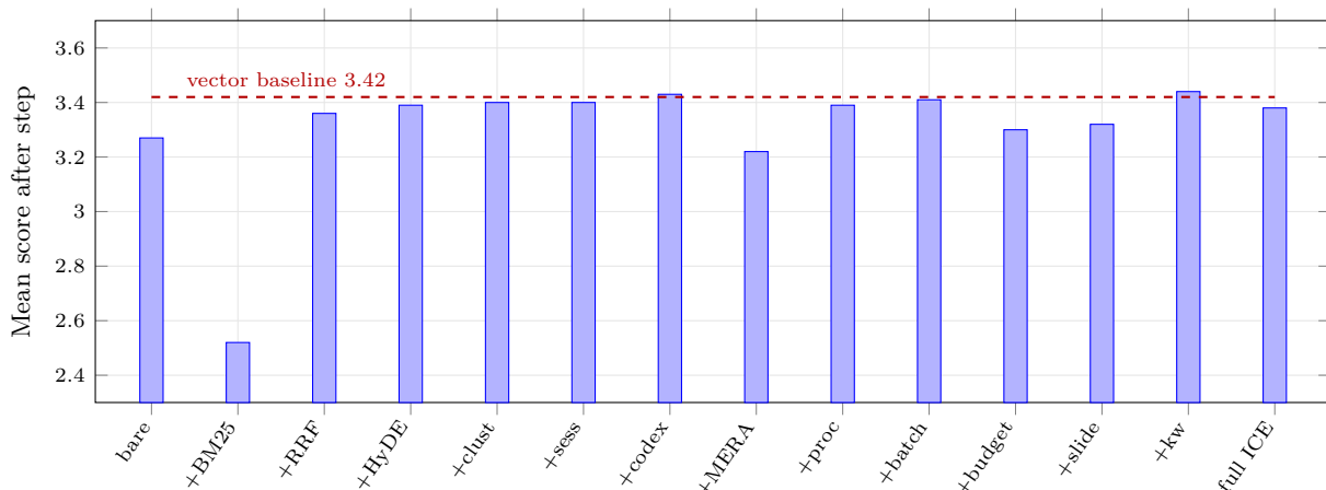
Figure 5: Feature ablation buildup (Dataset B, 67 probes, Experiment 3). Each bar is the cumulative mean score after adding one feature to all previous ones. The only two movements that clear a paired bootstrap CI are the +BM25 drop ( -0.74 ) and the +RRF recovery ( +0.82 ); all other step deltas are within noise, and several toggled features were non-functional at the snapshot (Section 8). The dashed line marks the single-leg vector baseline (3.42), which is not a step in the buildup; the full build finishes level with it.
