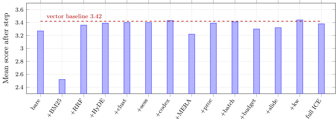
Figure 4: Feature ablation buildup (Dataset B, 67 probes). Each bar is the cumulative mean score after adding one feature to all previous ones. The only two movements clearing a paired bootstrap CI are the +BM25 drop and the +RRF recovery. The dashed line marks the single-leg vector baseline, which is not a buildup step; the full build finishes level with it.
