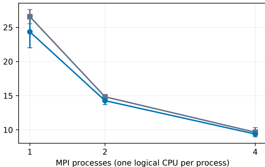
Multi-front churn, N=32 (35,937 DOFs)
