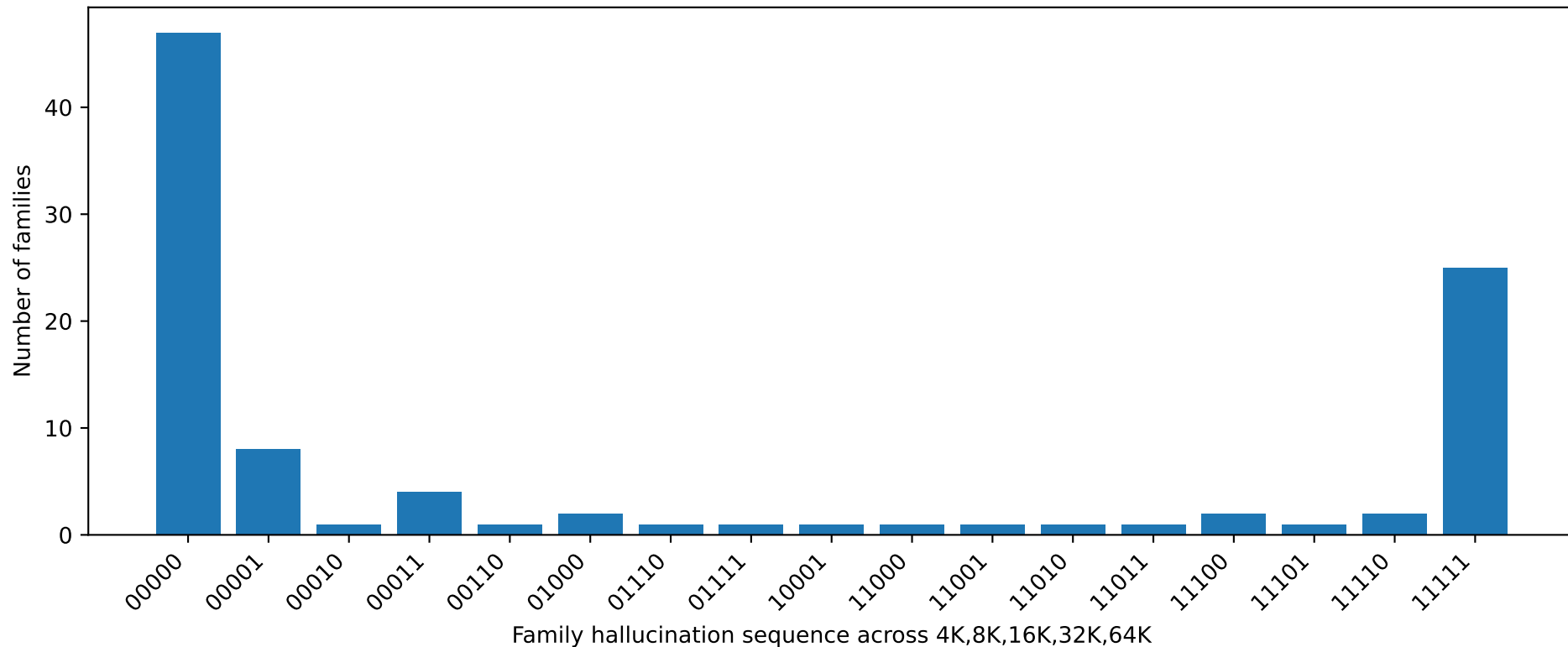
Family-Level Hallucination Transition Patterns
