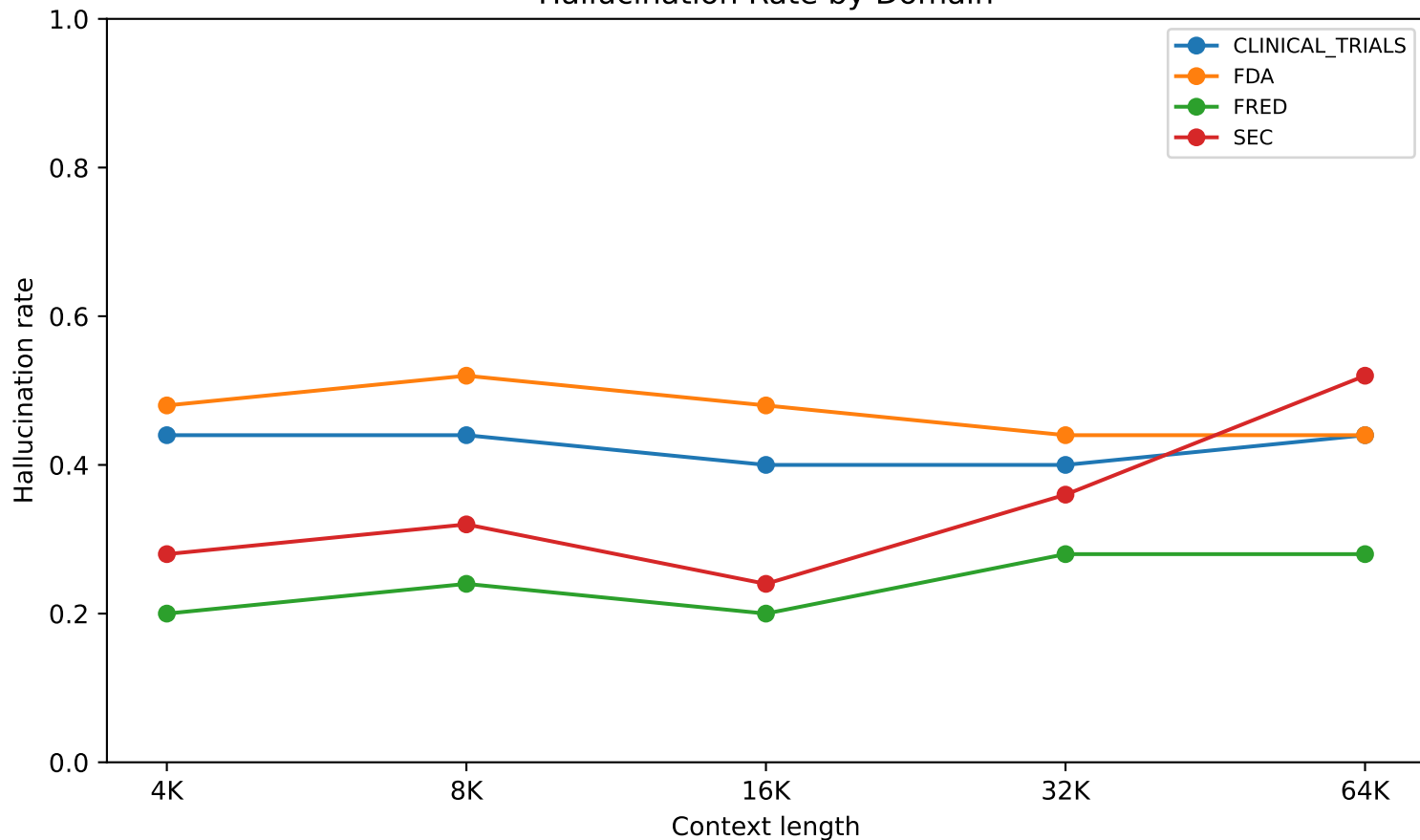
Hallucination Rate by Domain
