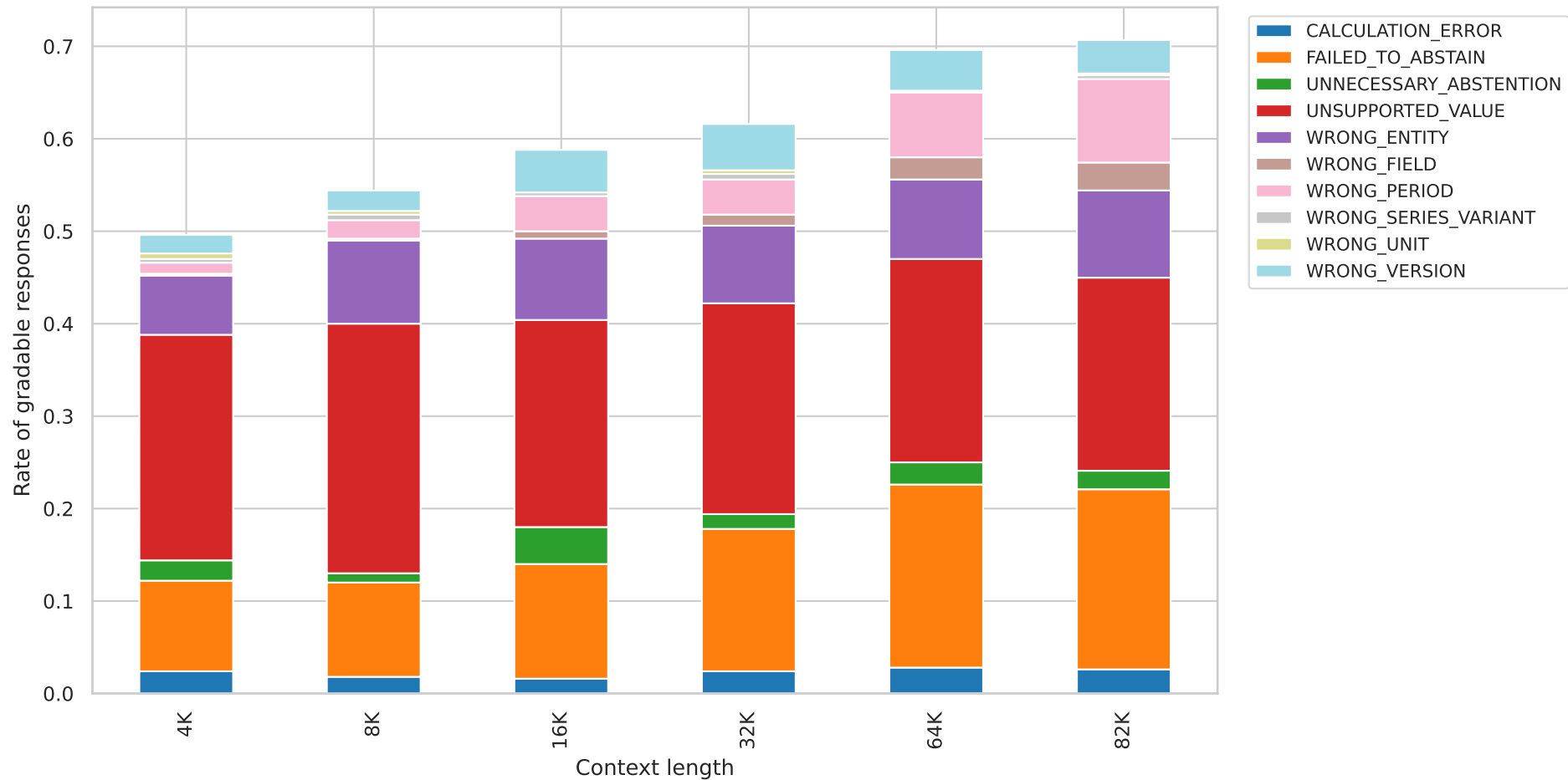
Error-type composition by context length
