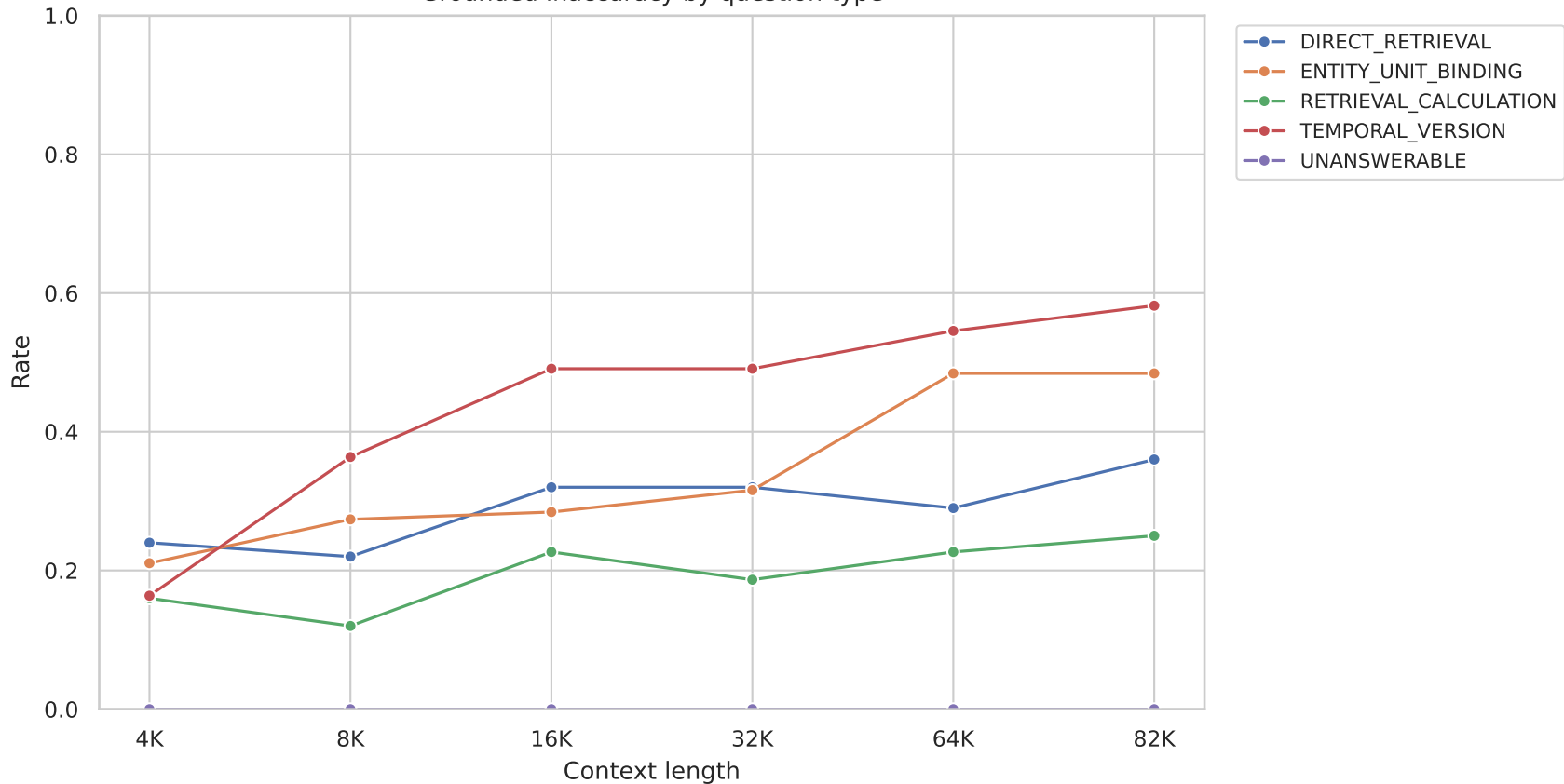
Grounded inaccuracy by question type
