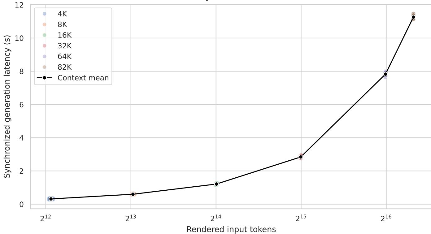
Inference latency vs rendered context tokens
