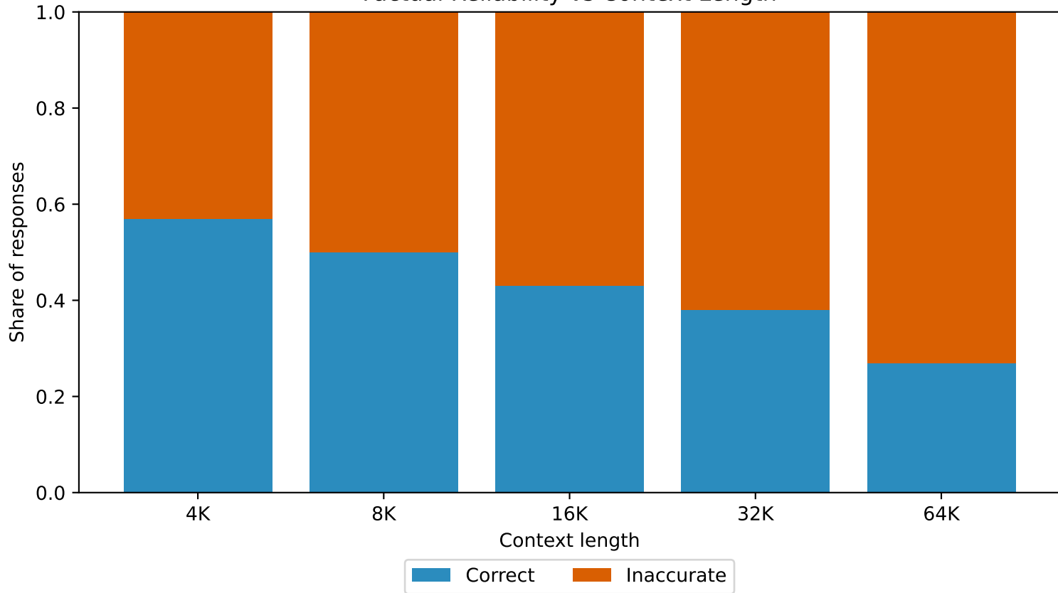
Factual Reliability vs Context Length
