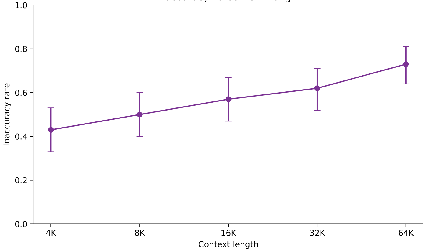
Inaccuracy vs Context Length
