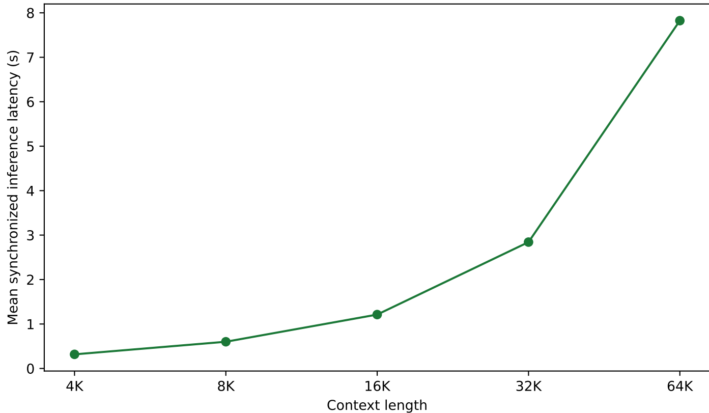
Inference Latency vs Context Length
