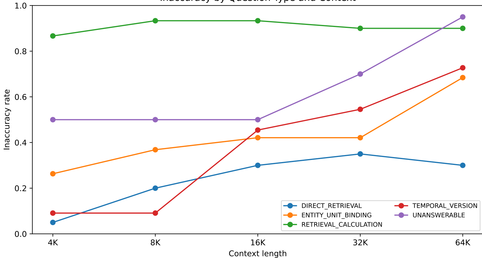
Inaccuracy by Question Type and Context
