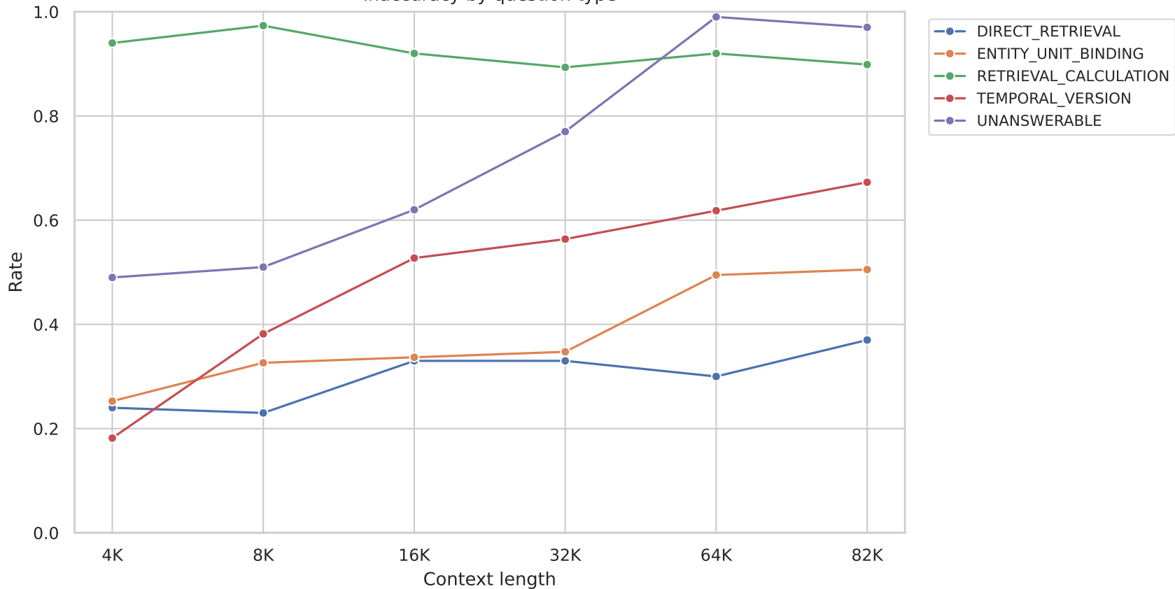
Inaccuracy by question type
