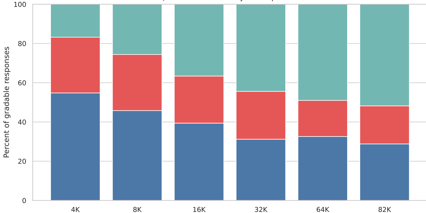
Qwen factual reliability decomposition
