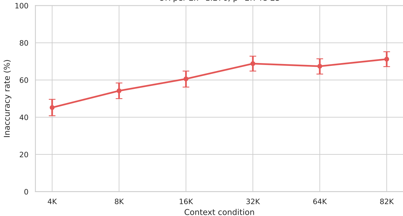
Qwen Inaccuracy rate (%) OR per 2x=1.276, p=2.74e-23
