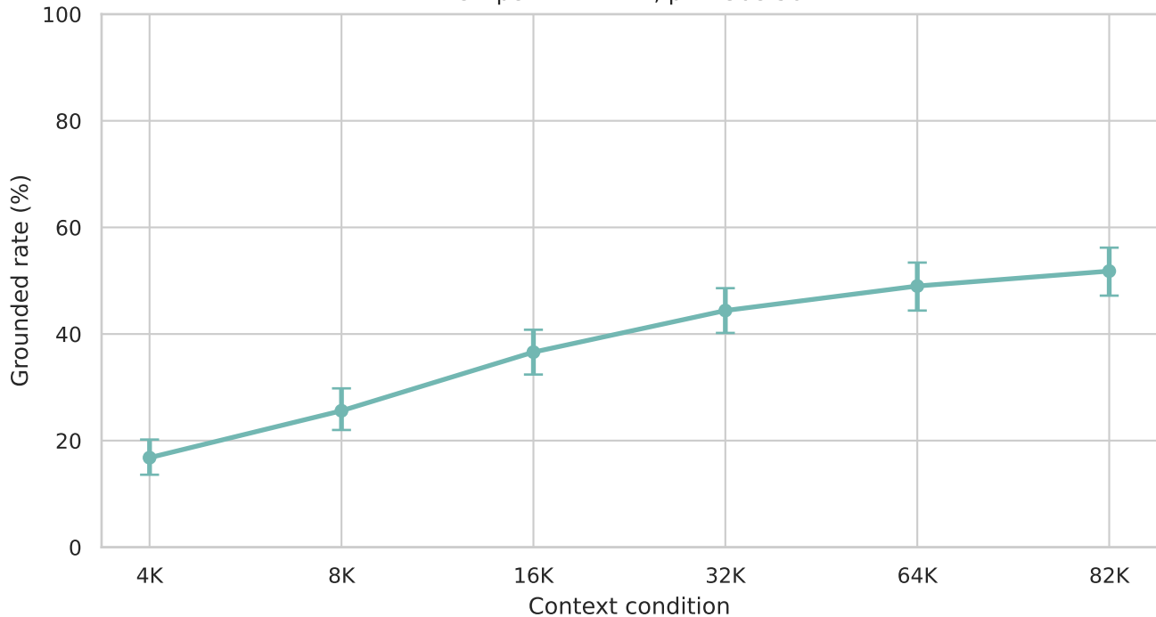
Qwen Grounded rate (%) OR per 2x=1.447, p=1.36e-56
