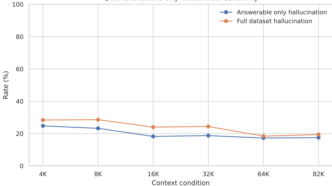
Qwen answerable-only hallucination sensitivity
