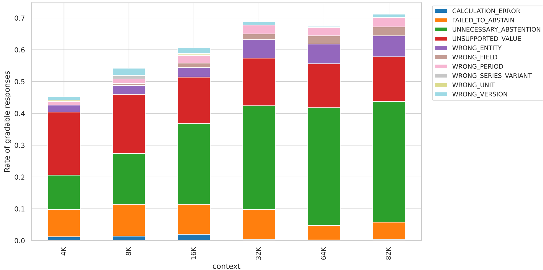
Qwen detailed error evolution
