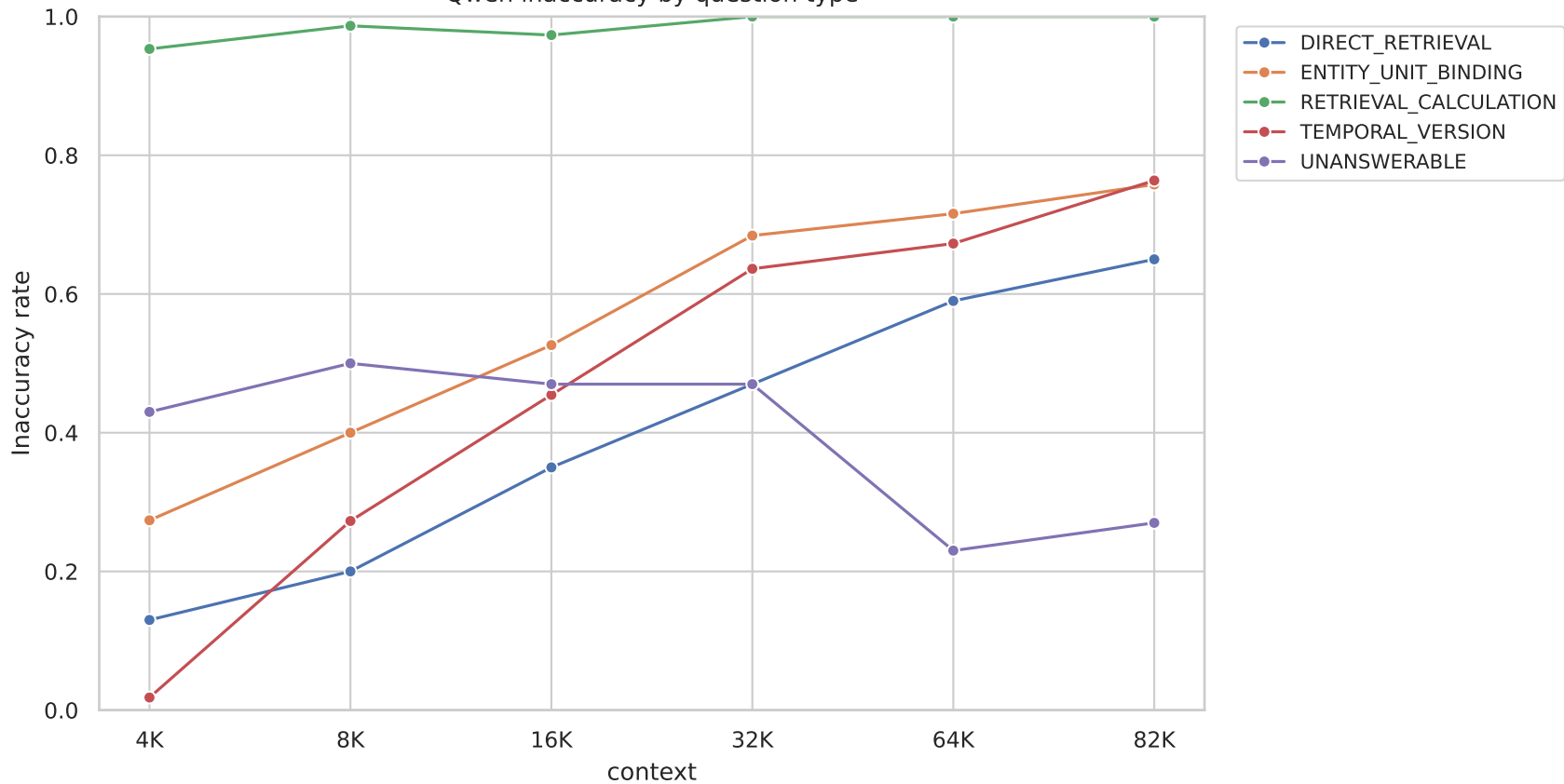
Qwen inaccuracy by question type
