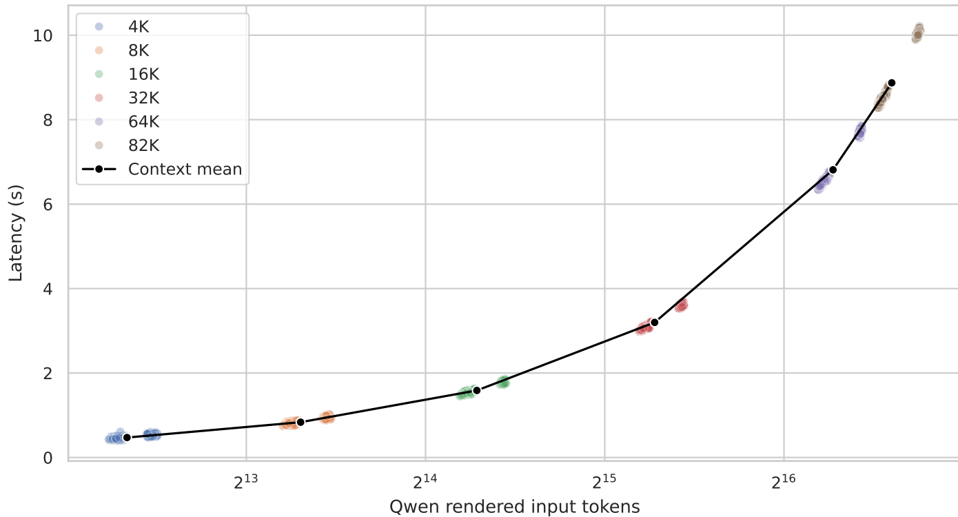
Qwen latency vs rendered context tokens
