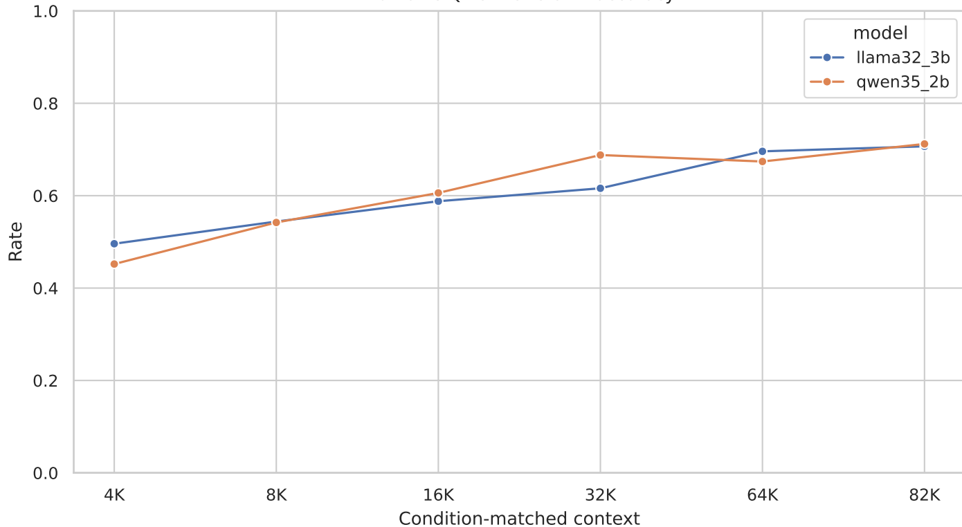
Llama vs Qwen: Overall inaccuracy
