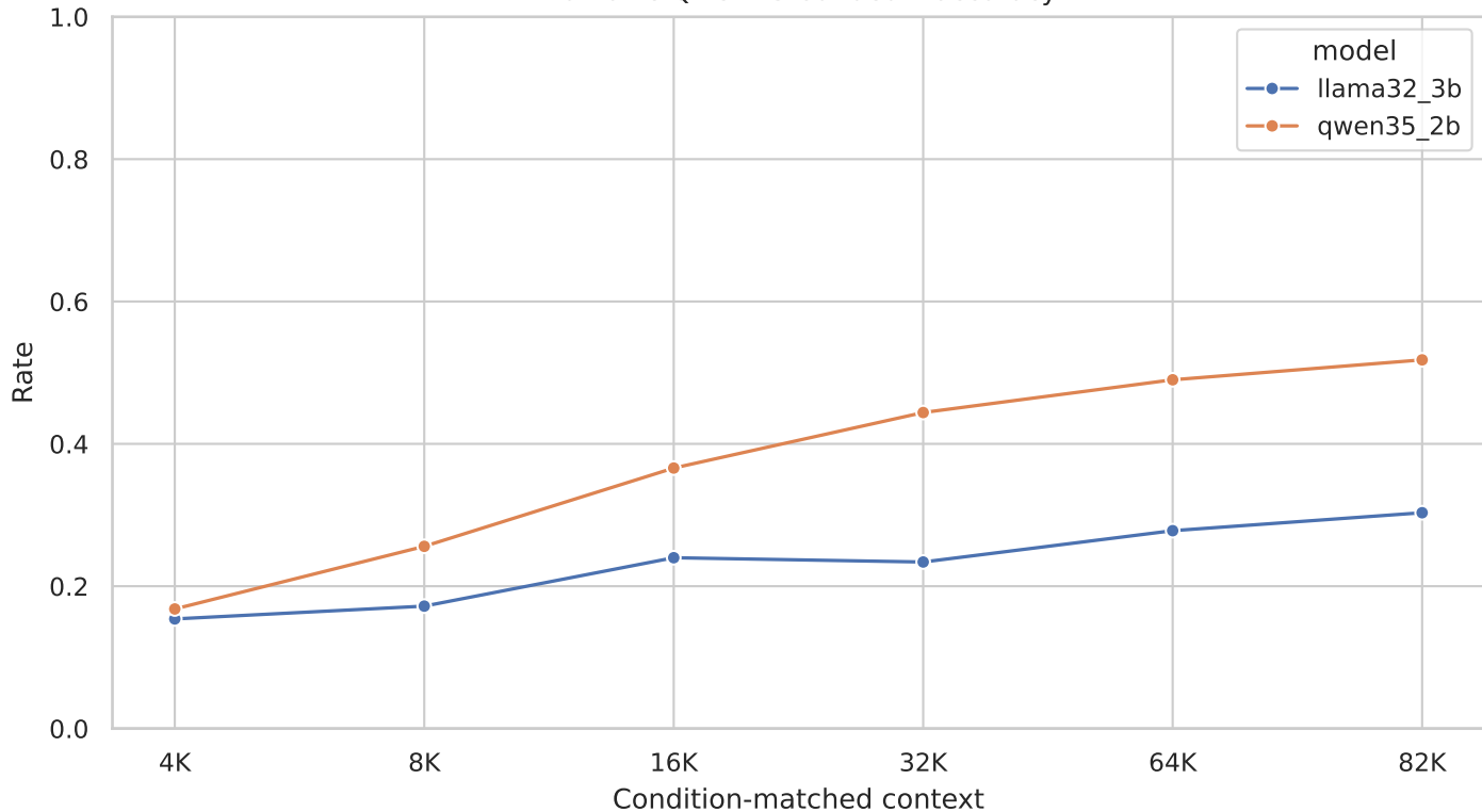
Llama vs Qwen: Grounded inaccuracy
