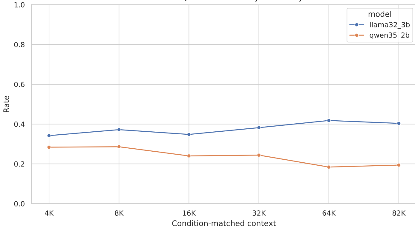
Llama vs Qwen: Hallucinatory inaccuracy
