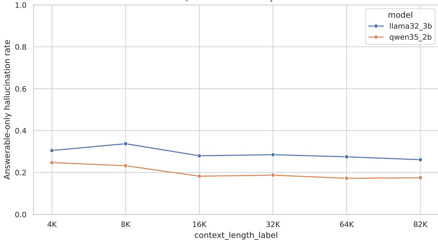
Llama vs Qwen answerable-only hallucination
