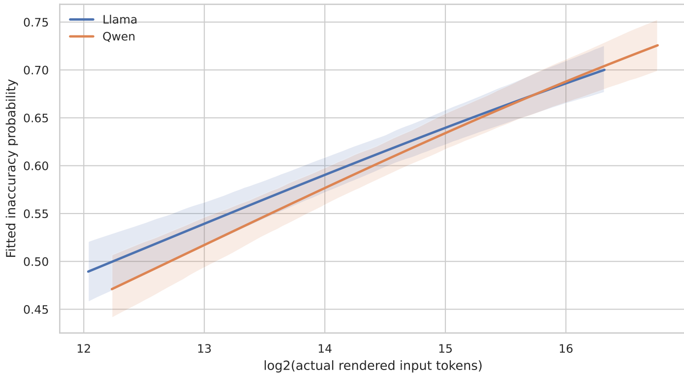
Cross-model slope comparison
