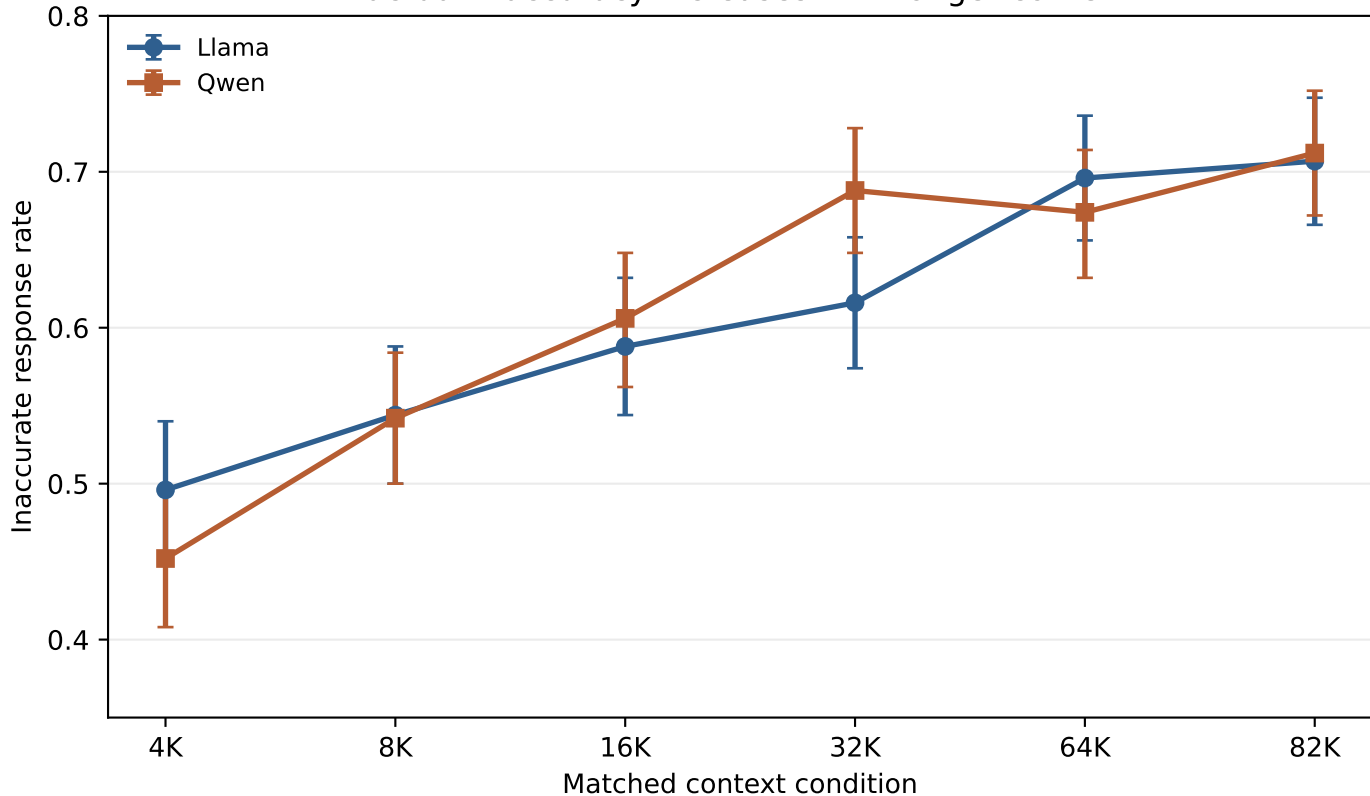
Factual inaccuracy increases with longer context
