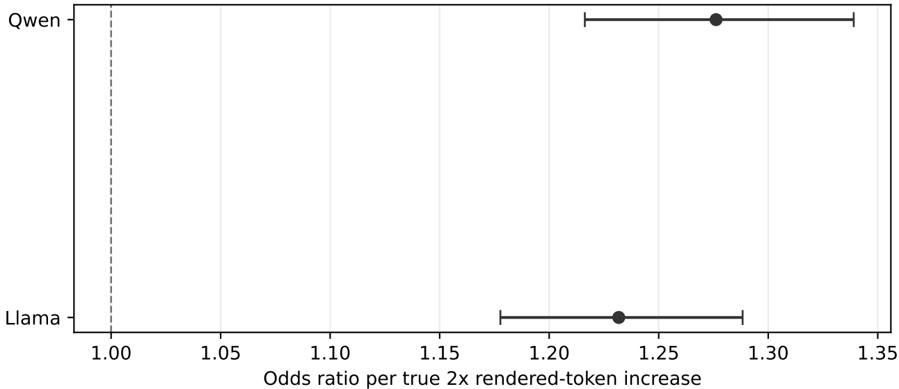
Model-specific degradation slopes
