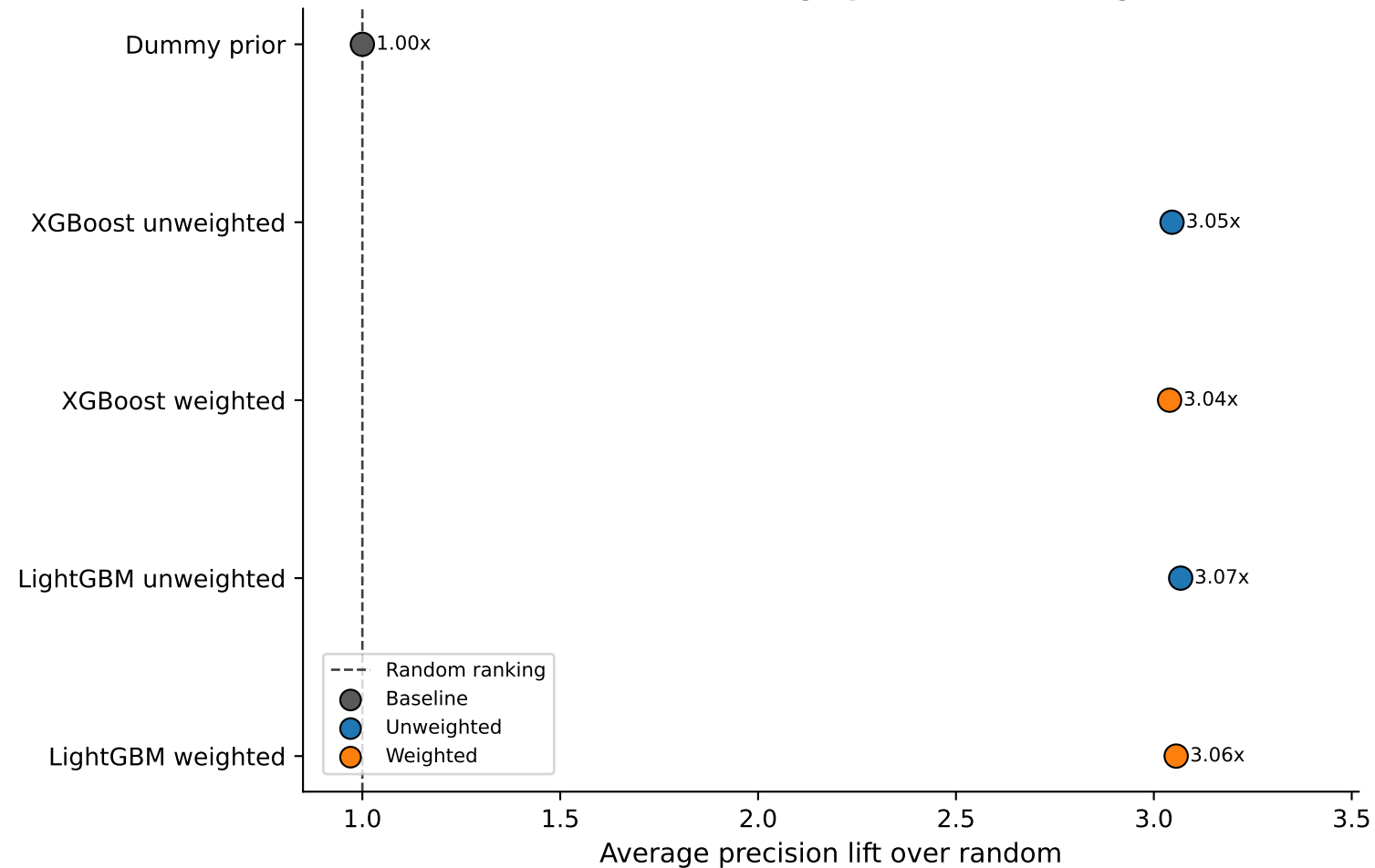
Validation average precision ranking
