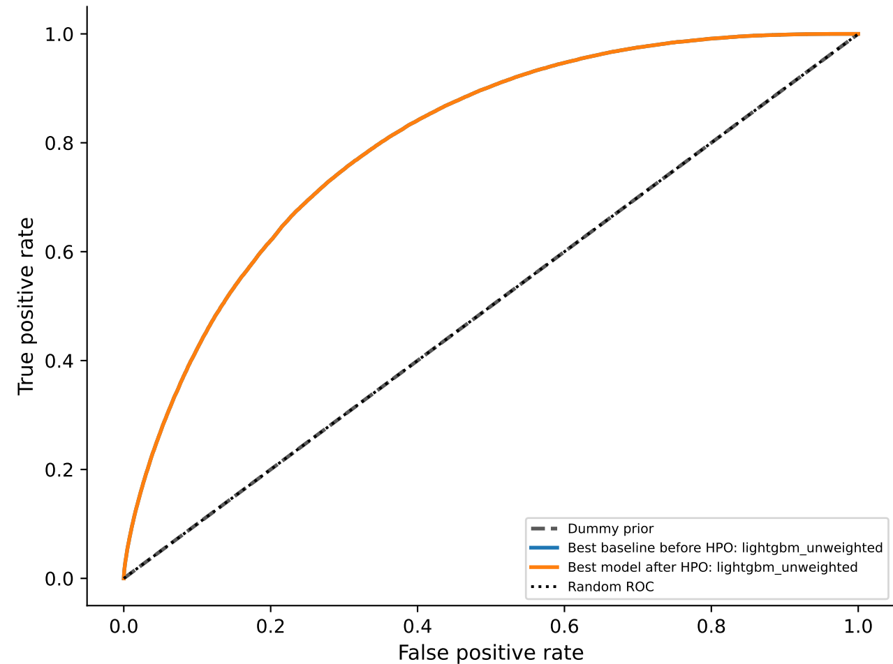
Validation ROC curves
